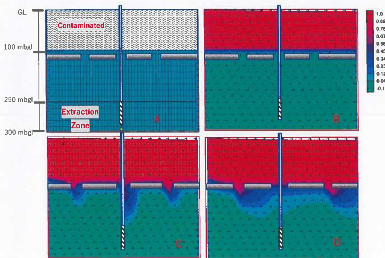
Figure 5. Simulation of contaminant transport to deeper depths with time (Scenario 3).
