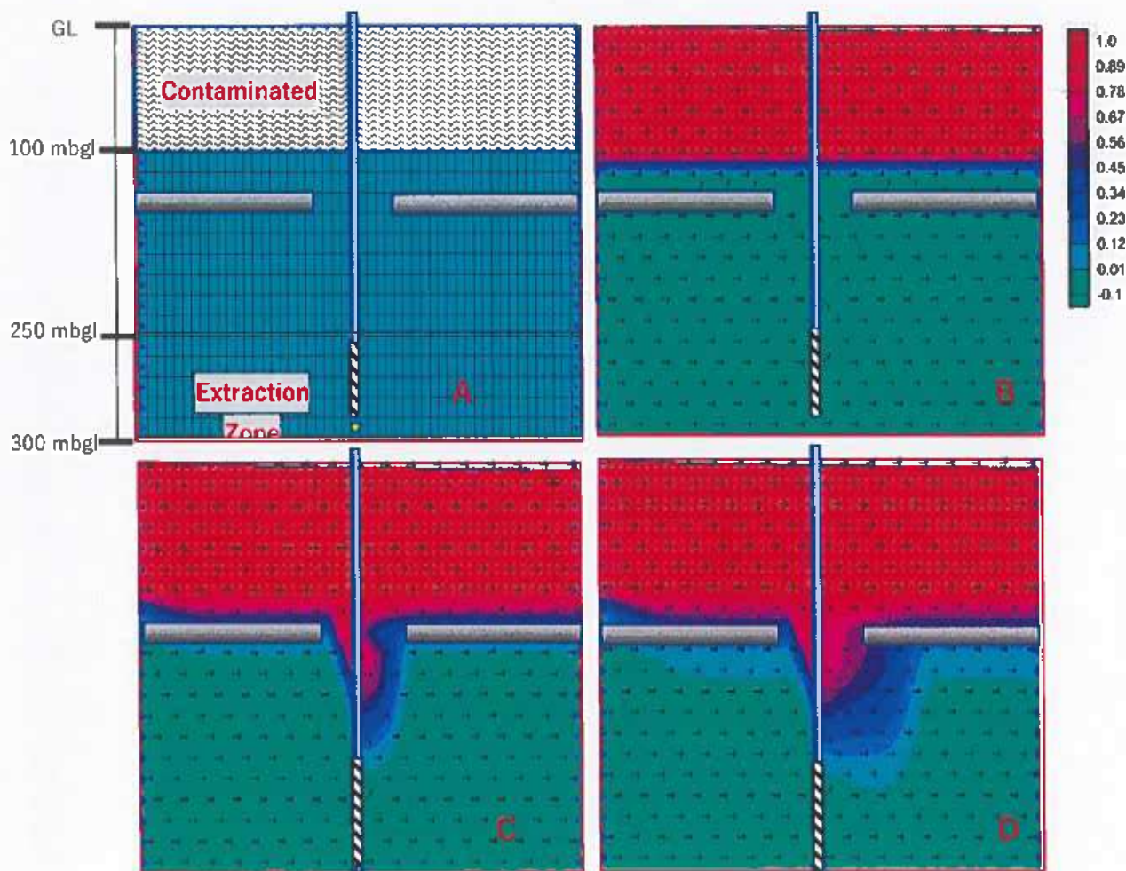
Figure 4. Simulation of contaminant transport to deeper depths with time (Scenario 2)
