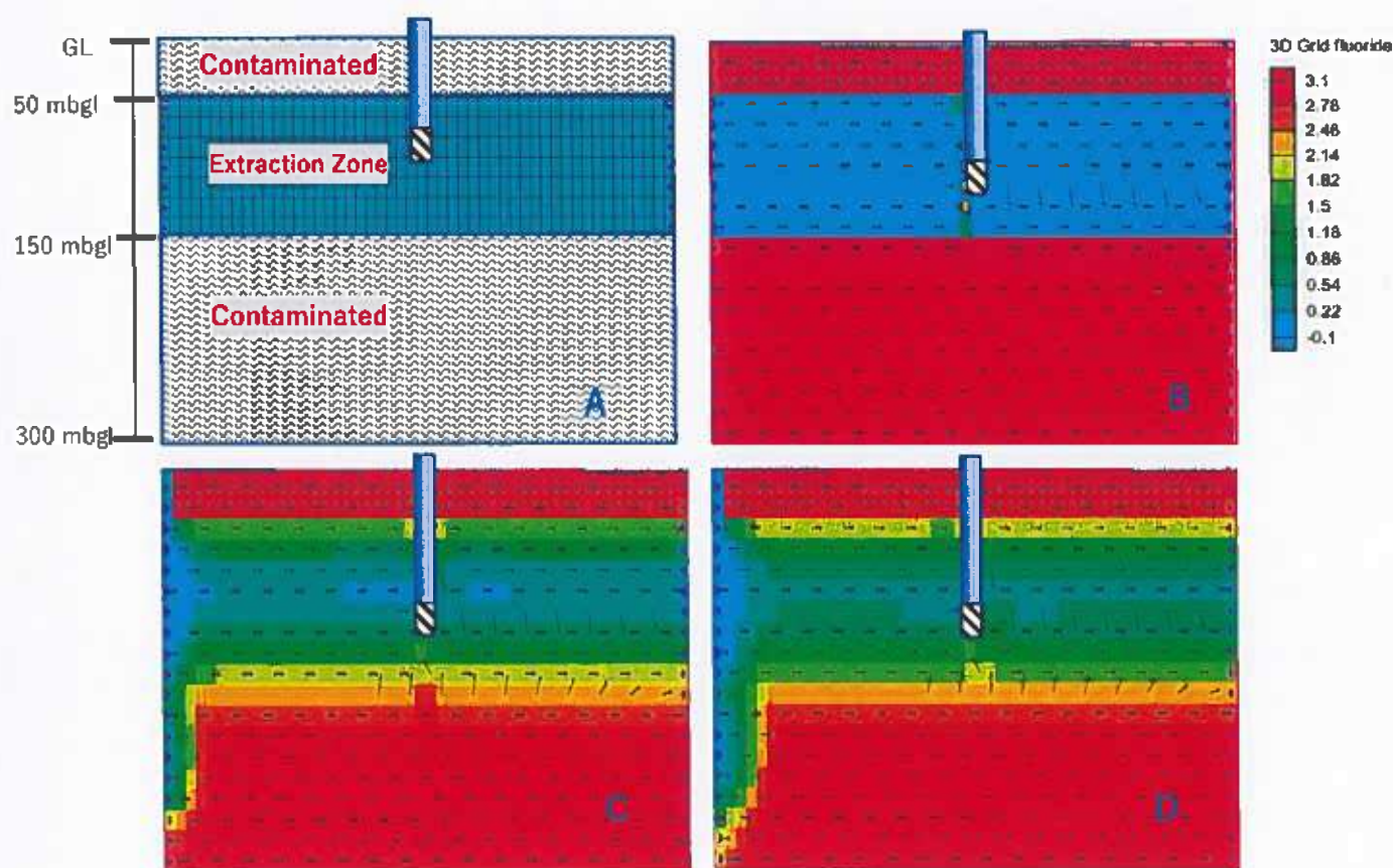
Figure 8. Contaminant transport simulation in Unnao.
