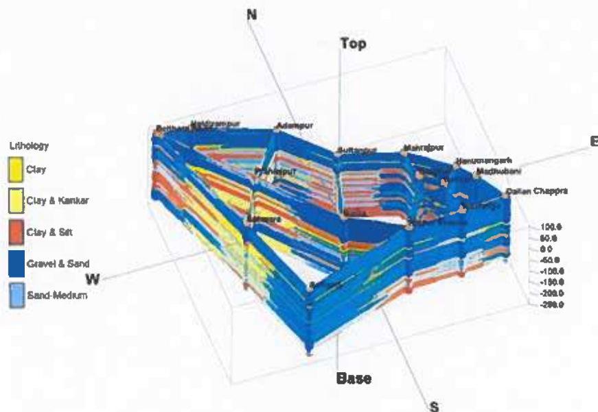
Figure 1. Lithological Fence diagram of Ballia district (NAQUIM Report 2017)
