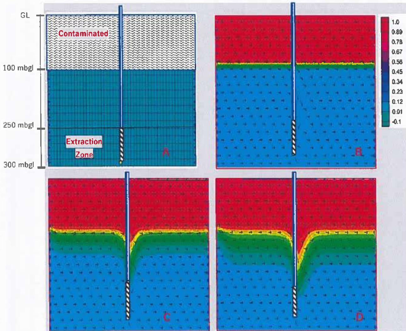
Figure 3. Simulation of contaminant transport to deeper depths with time (Scenario 1).
