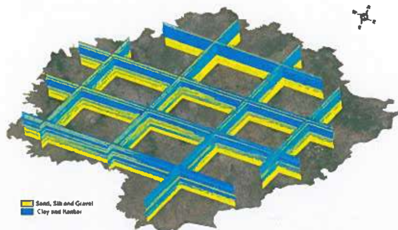
Figure 6. Lithological Fence diagram of Unnao district (NAQUIM Report 2017)
