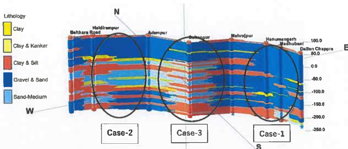
Figure 2. Basis of lithological configuration in Ballia case study (NAQUIM Report 2017)
